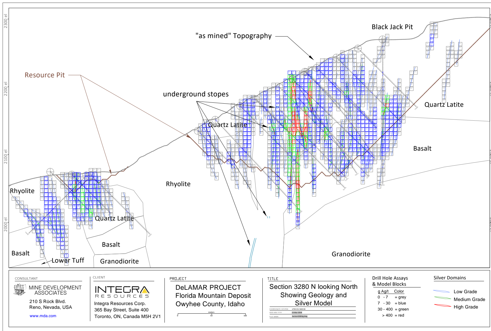
Figure 14.20 Cross Section 3280 N Showing Florida Mountain Block-Model Silver Grades
