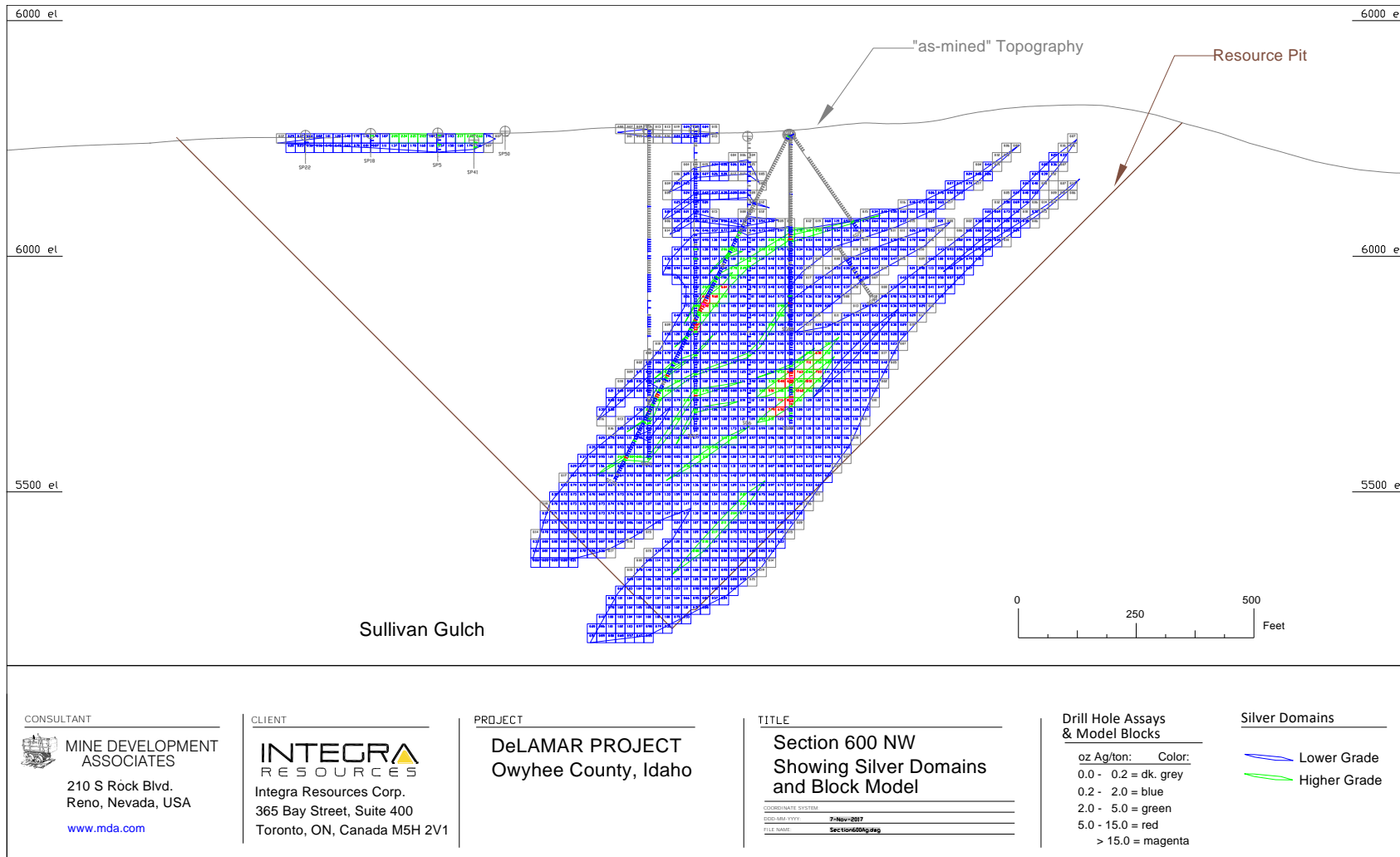
Figure 14.12 Cross Section 600 NW Showing Sullivan Gulch Block-Model Silver Grades
