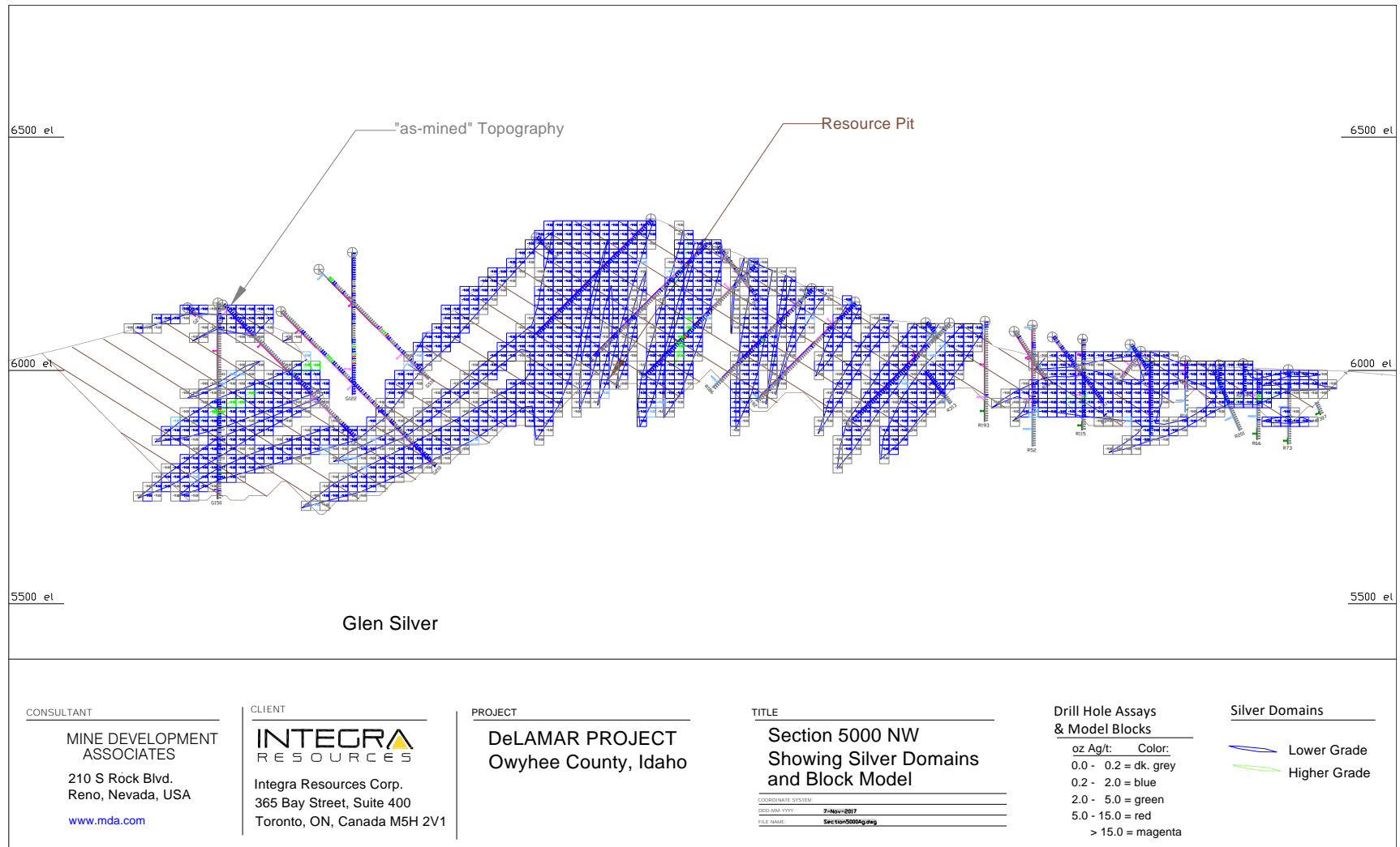
Figure 14.16 Cross Section 5000 NW Showing Glen Silver Block-Model Silver Grades
