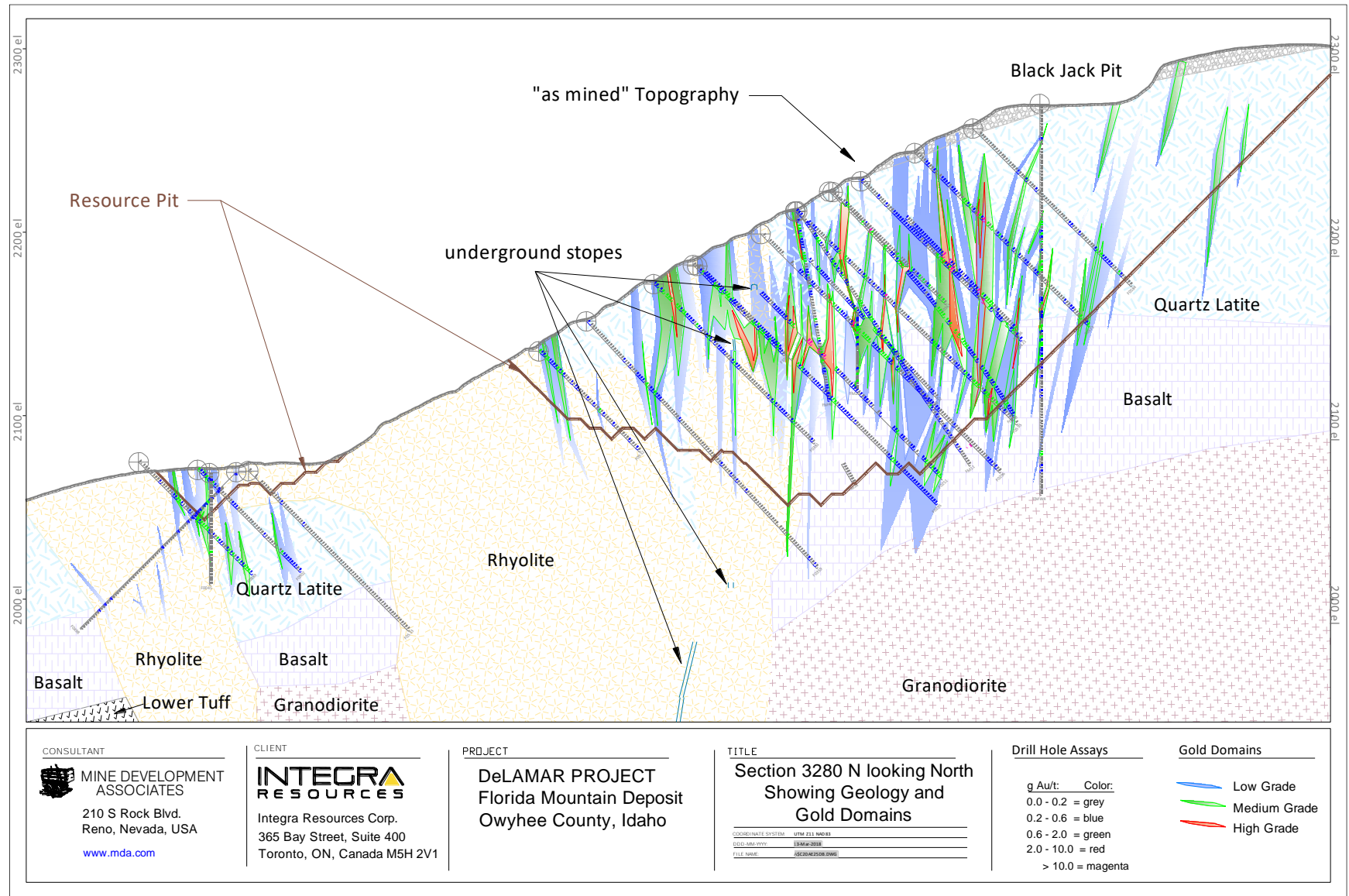
Figure 14.9 Cross Section 3280 N, Geology and Gold Domains for the Florida Mountain Area
