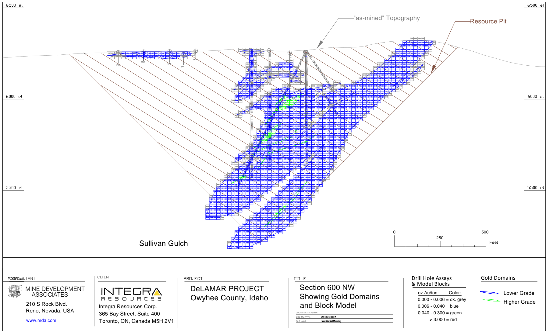
Figure 14.11 Cross Section 600 NW Showing Sullivan Gulch Block-Model Gold Grades
