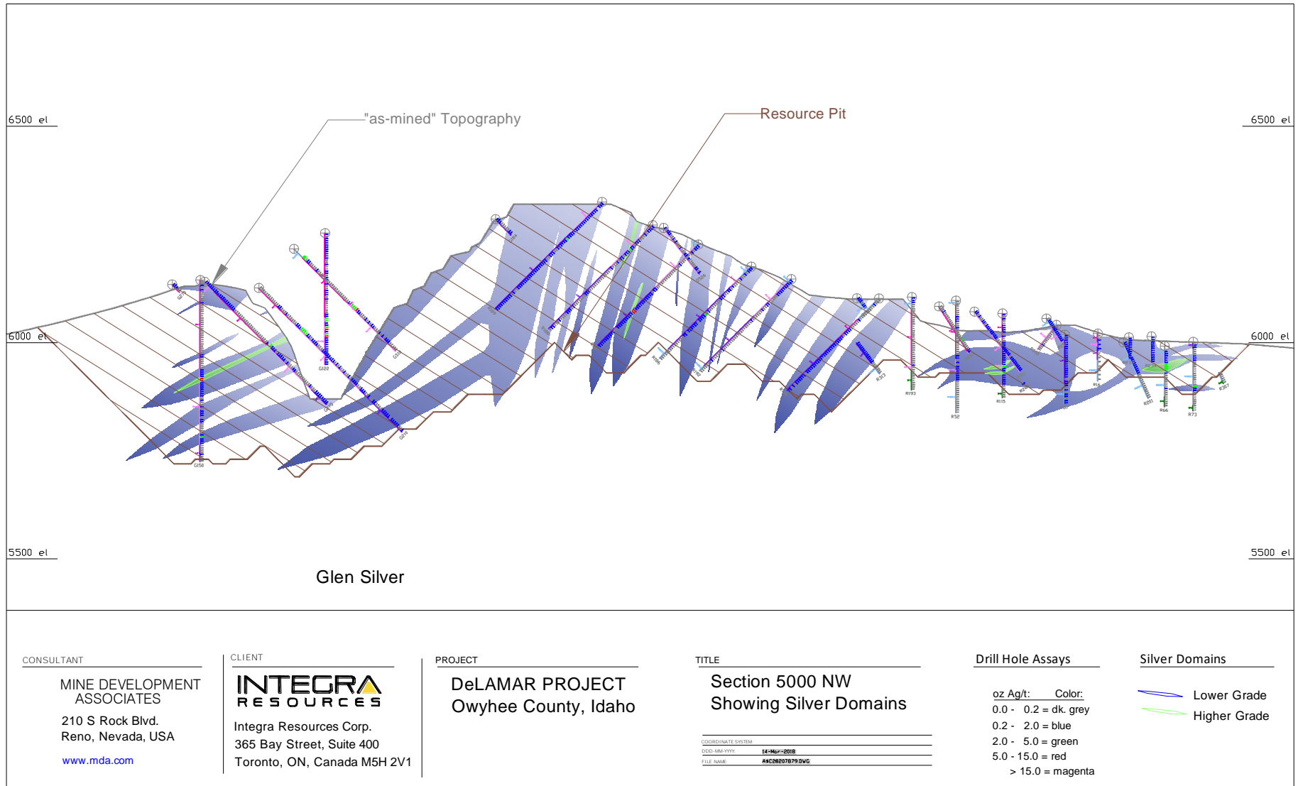
Figure 14.6 Glen Silver Cross Section 5000 NW Showing Silver Domains
