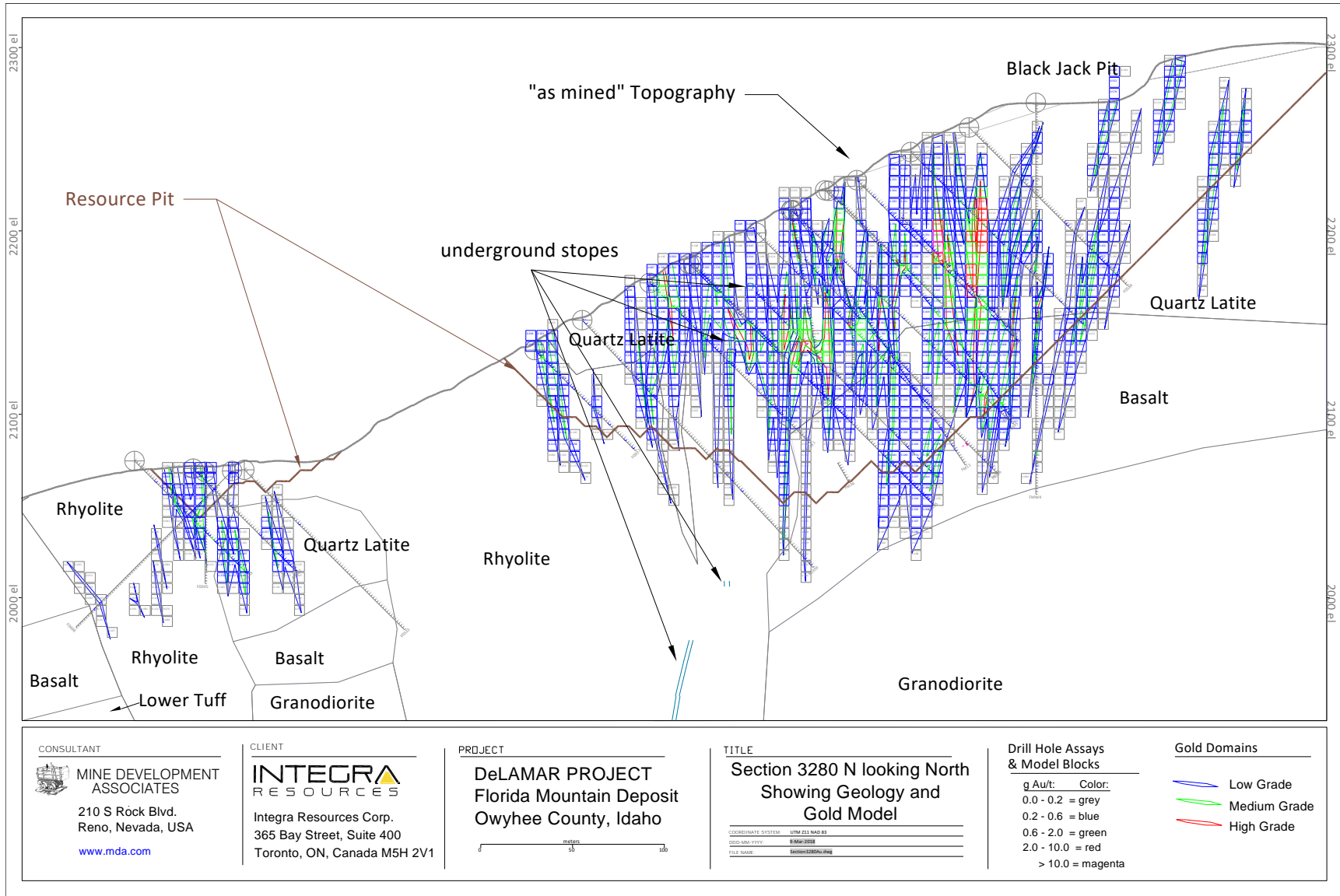
Figure 14.19 Cross Section 3280 N Showing Florida Mountain Block-Model Gold Grades
