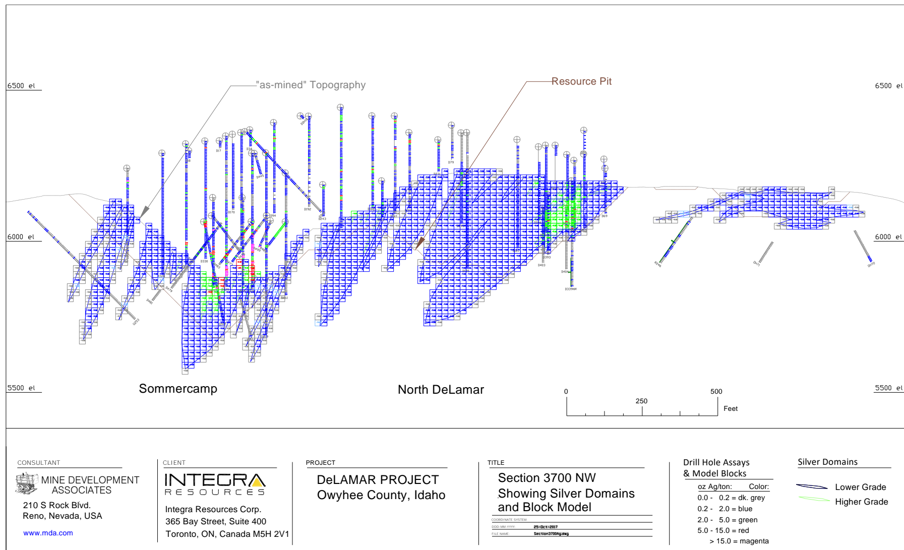
Figure 14.14 Cross Section 3700 NW, Sommercamp – Regan and N. DeLamar Block-Model Silver Grades
