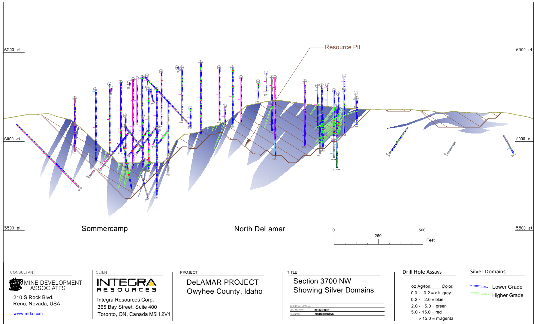
Figure 14.4 Cross Section 3700 NW, Sommercamp – Regan and N. DeLamar Silver Domains
