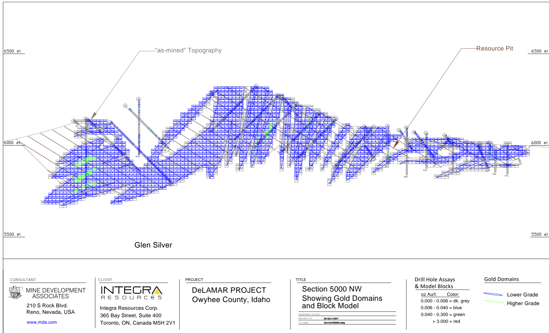
Figure 14.15 Cross Section 5000 NW Showing Glen Silver Block-Model Gold Grades
