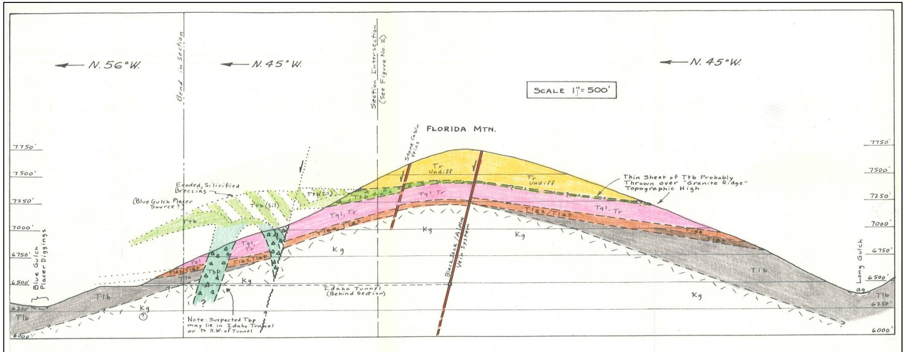
Figure 7.8 Schematic Florida Mountain Cross Section (Looking Northeast) (from Lindberg, 1985)
