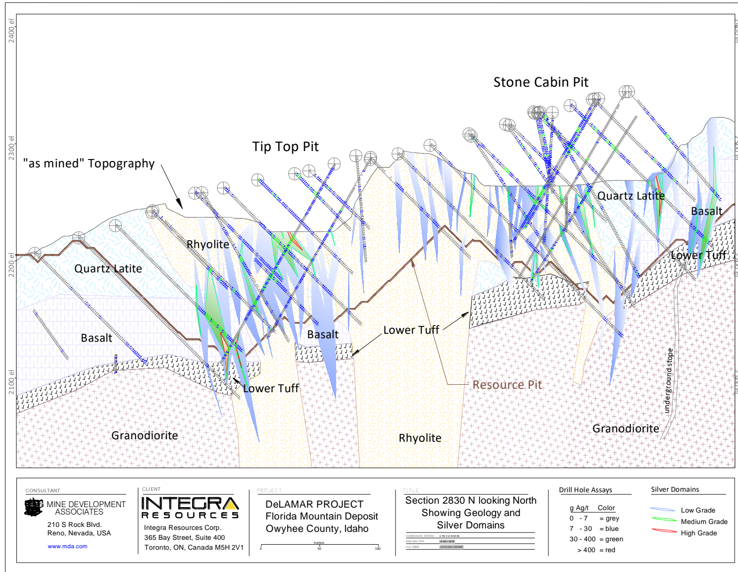
Figure 14.8 Cross Section 2830 N, Geology and Silver Domains for the Florida Mountain Area
