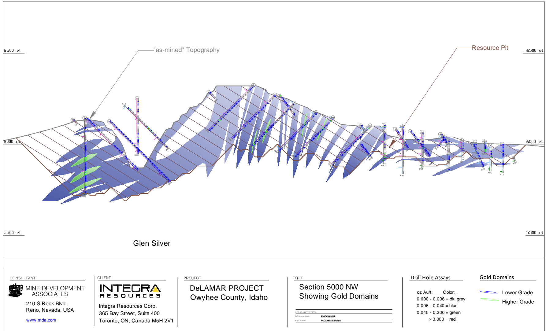
Figure 14.5 Glen Silver Cross Section 5000 NW Showing Gold Domains
