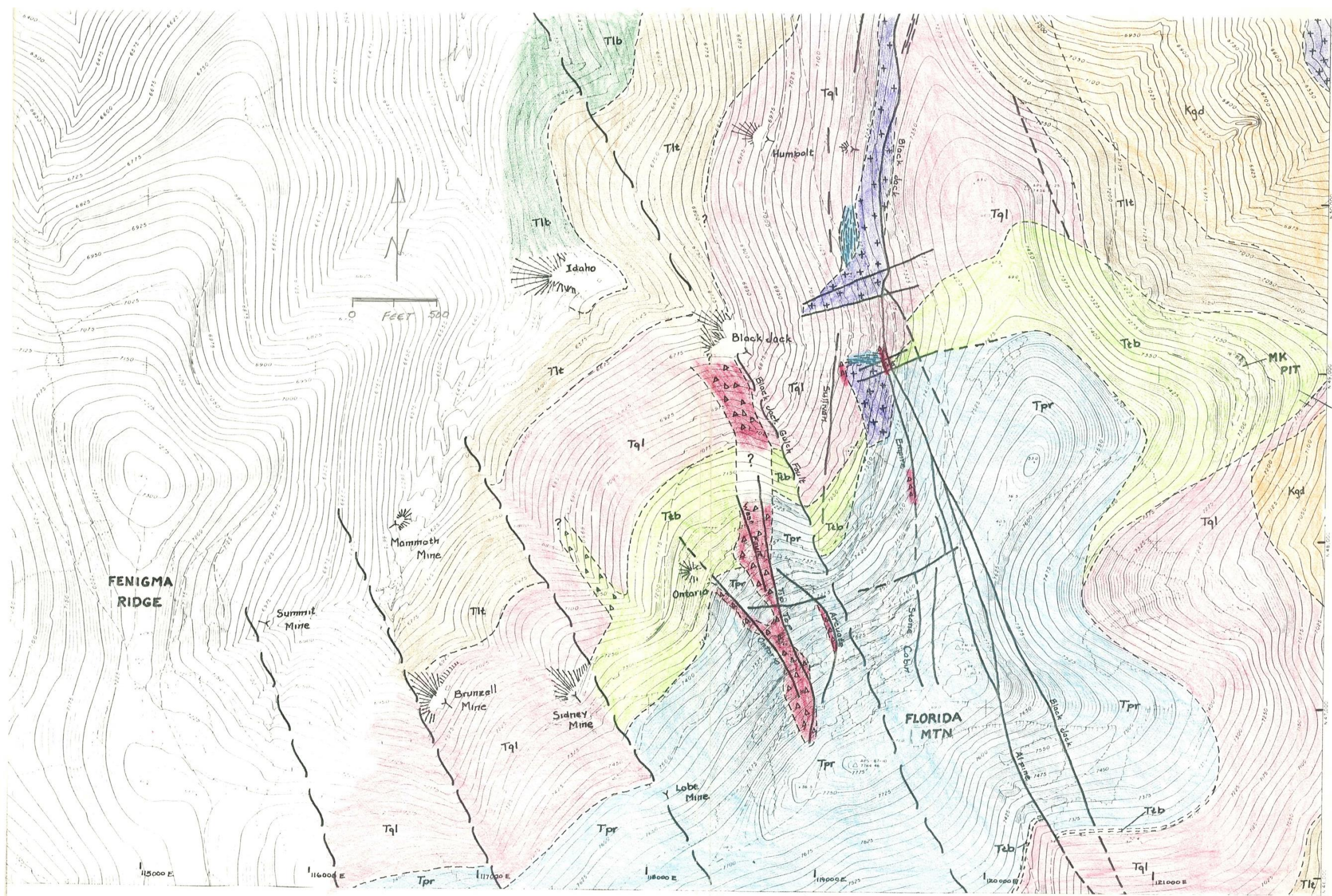
Figure 7.6 Geologic Map of Florida Mountain (from Porterfield and Moss, 1988)
