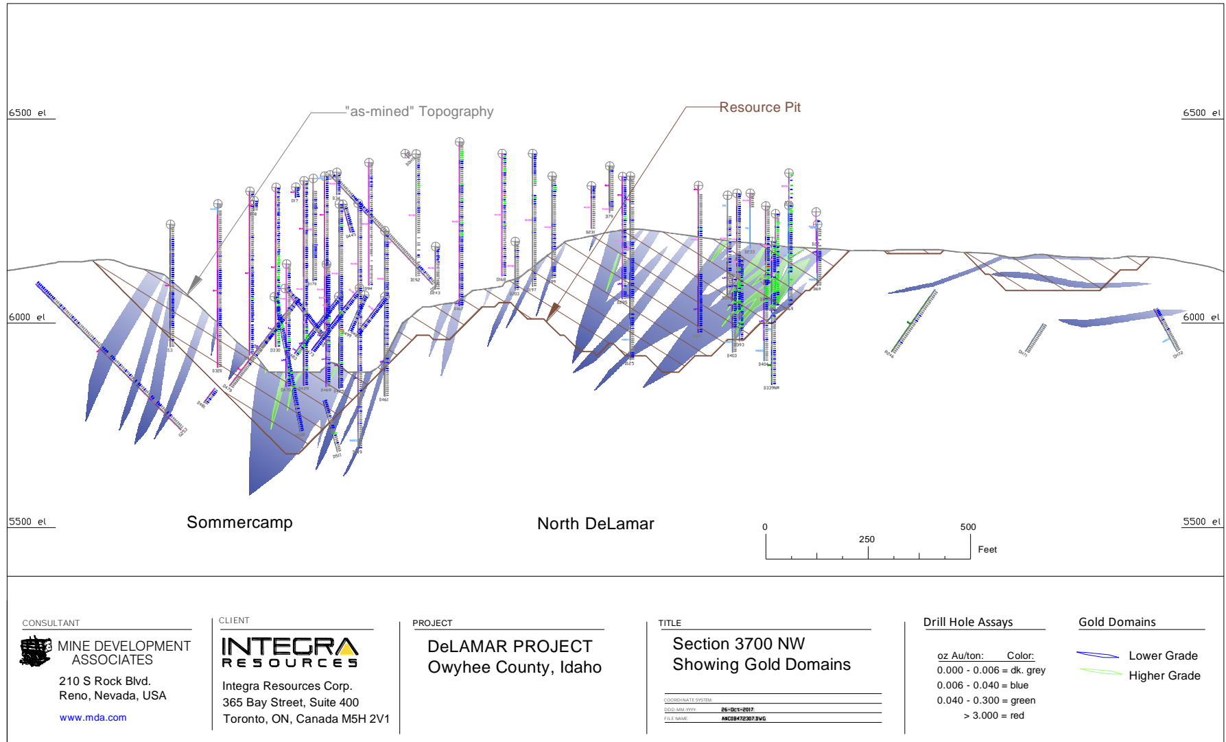
Figure 14.3 Cross Section 3700 NW, Sommercamp – Regan and N. DeLamar Gold Domains
