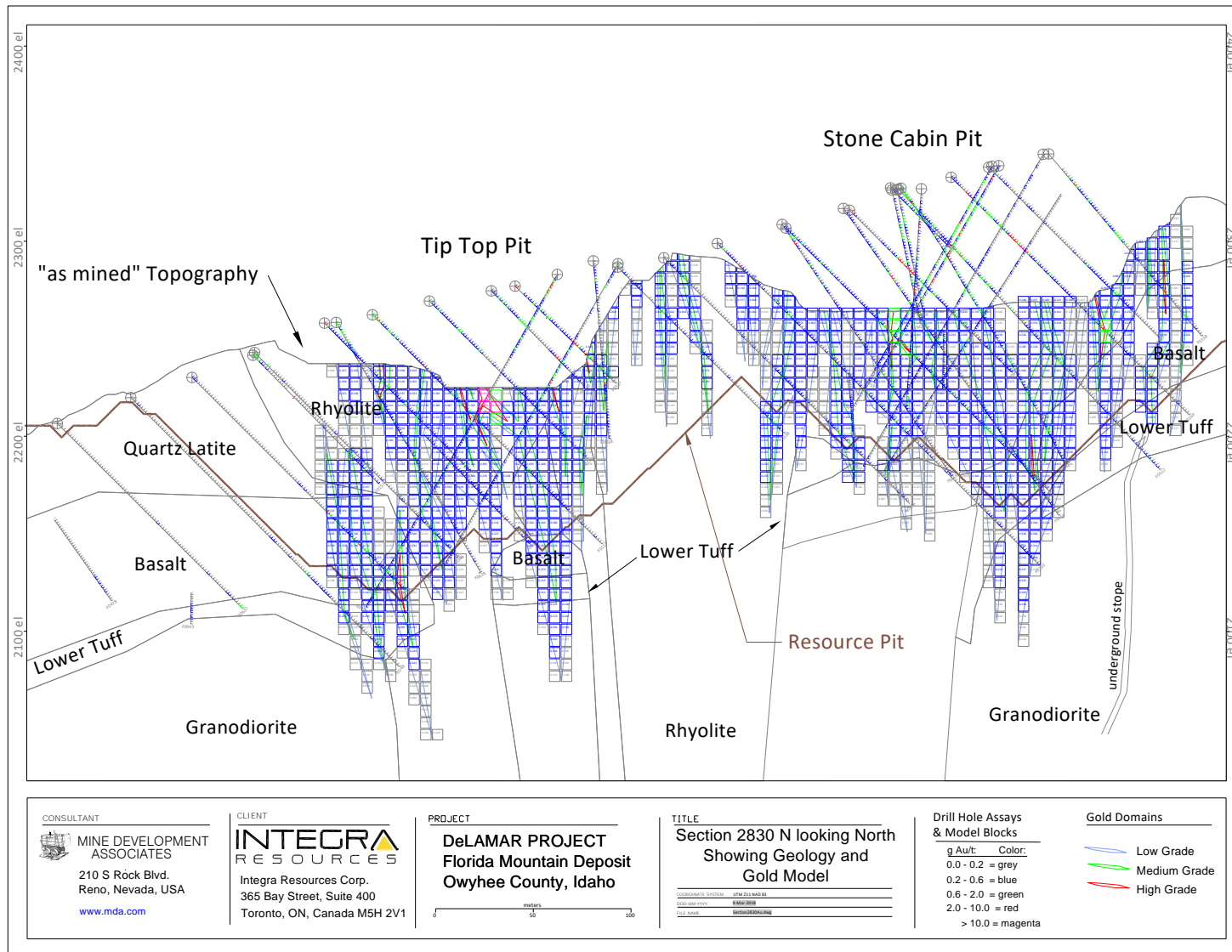
Figure 14.17 Cross Section 2830 N Showing Florida Mountain Block-Model Gold Grades
