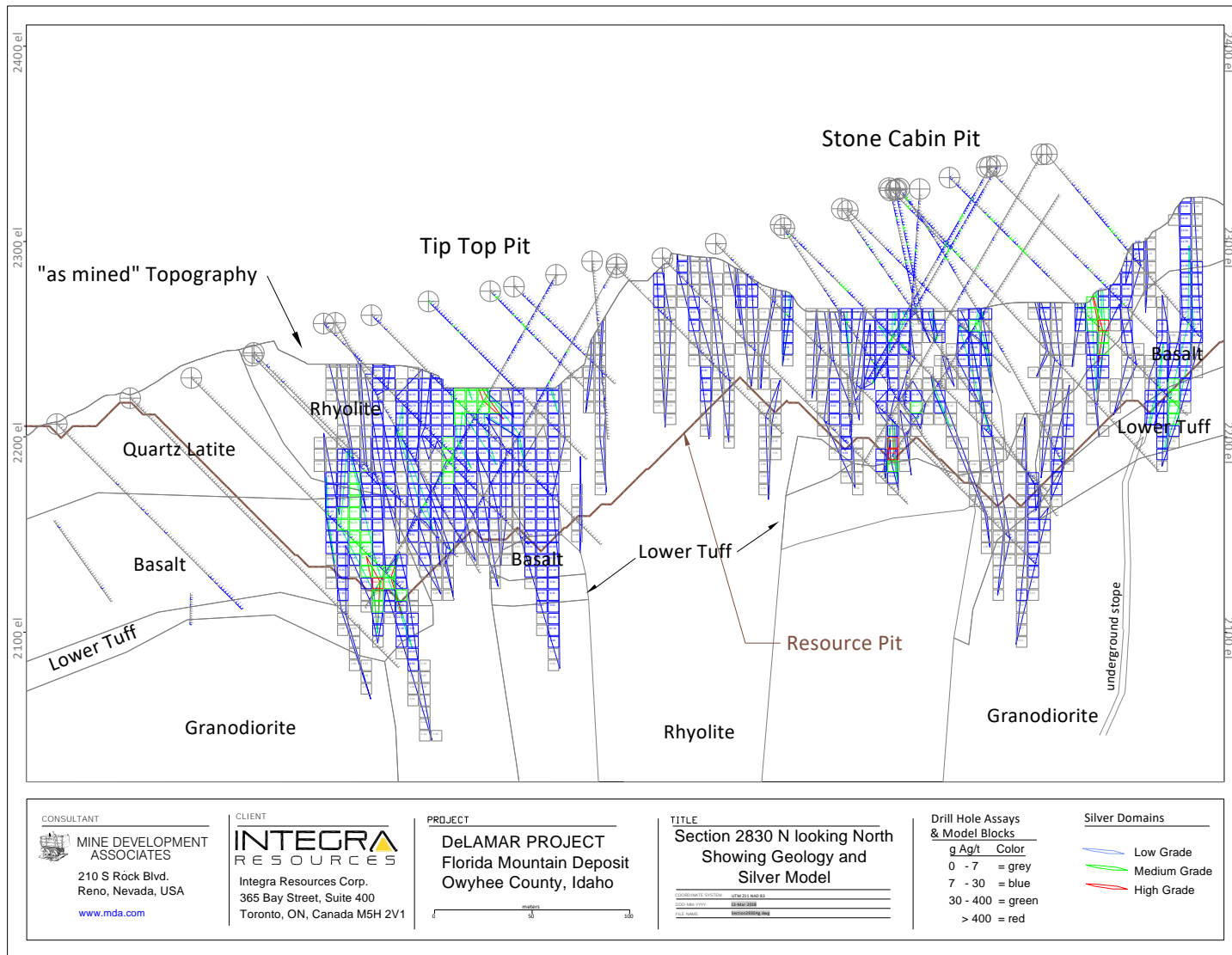
Figure 14.18 Cross Section 2830 N Showing Florida Mountain Block-Model Silver Grades
