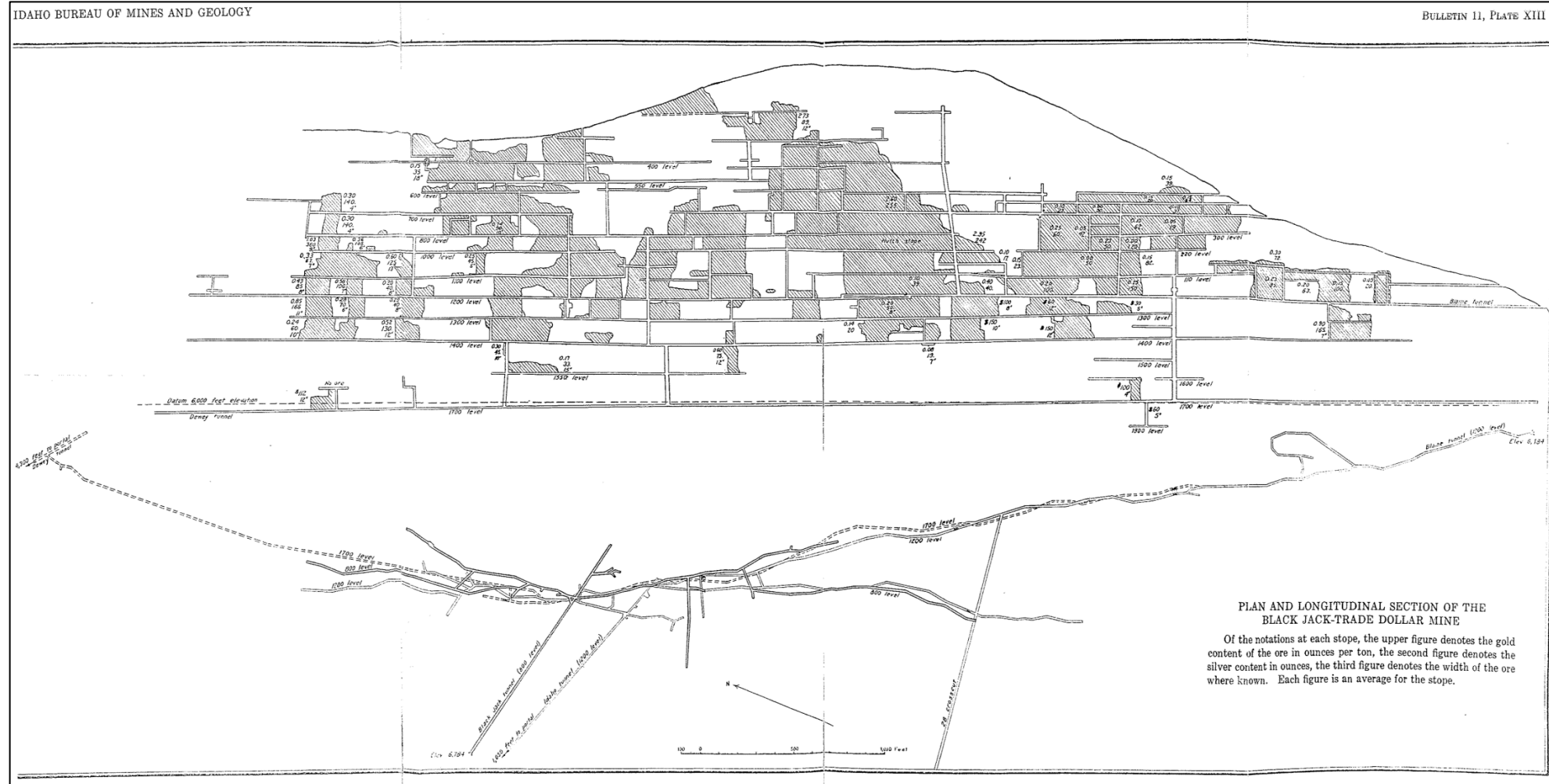
Figure 7.10 Longitudinal Section of the Black Jack – Trade Dollar Mine (from Piper and Laney, 1926)
