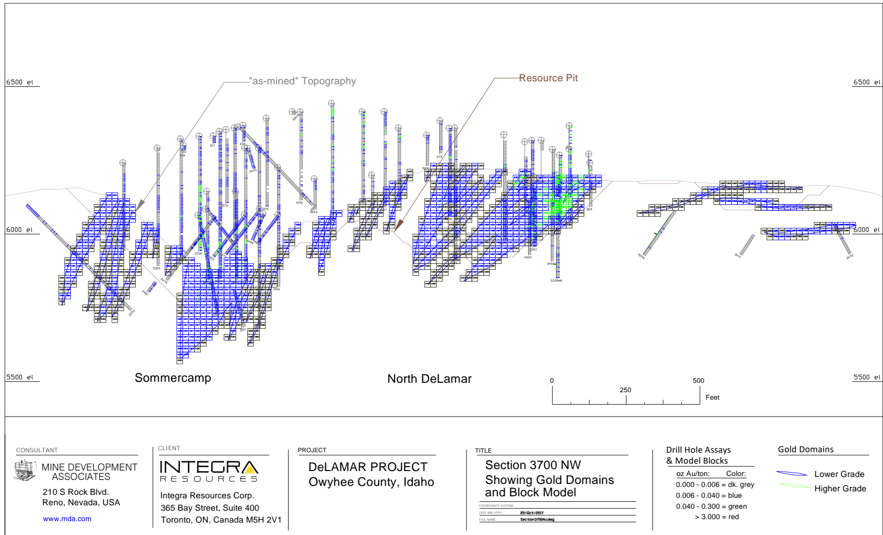
Figure 14.13 Cross Section 3700 NW, Sommercamp – Regan and N. DeLamar Block-Model Gold Grades
