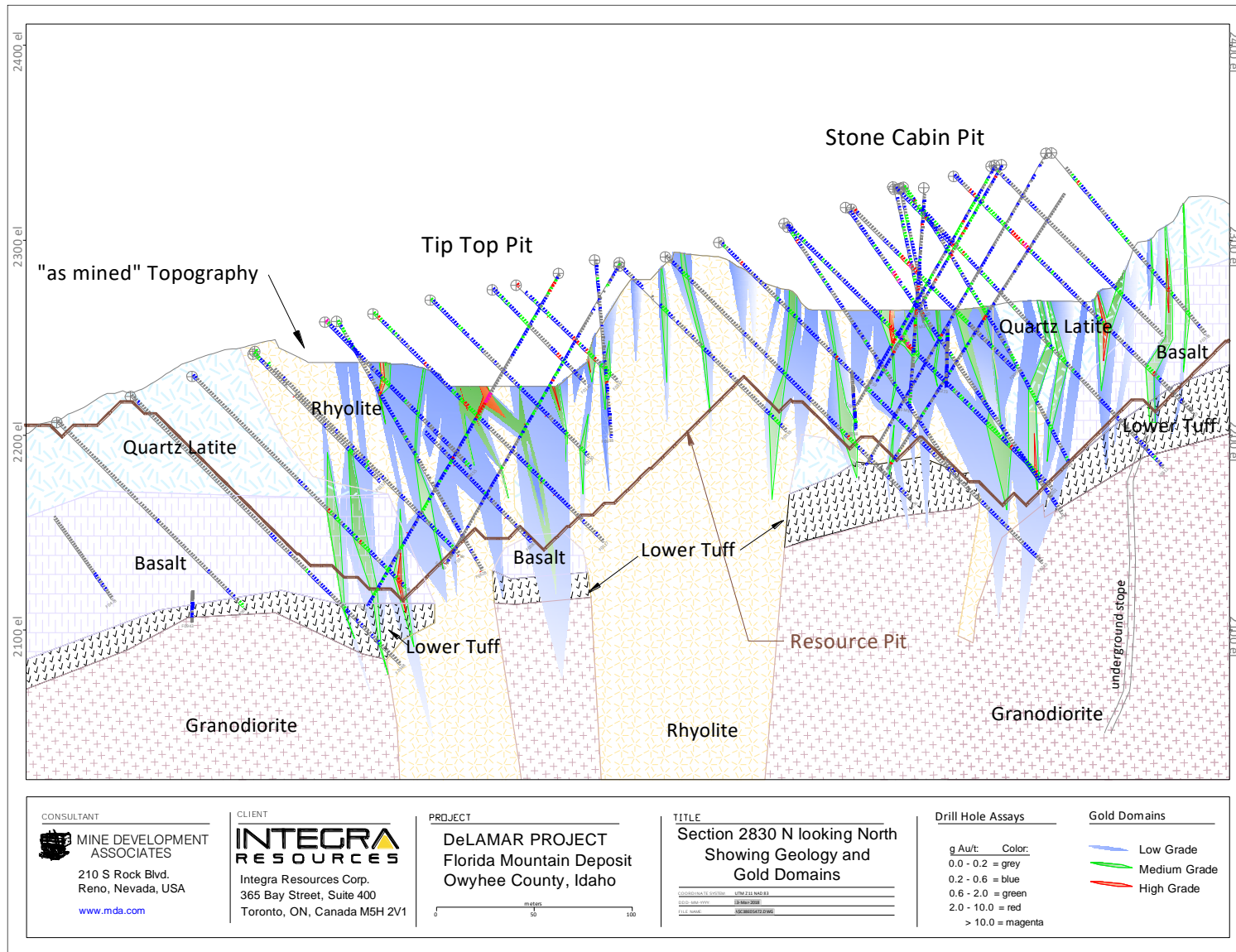
Figure 14.7 Cross Section 2830 N, Geology and Gold Domains for the Florida Mountain Area
