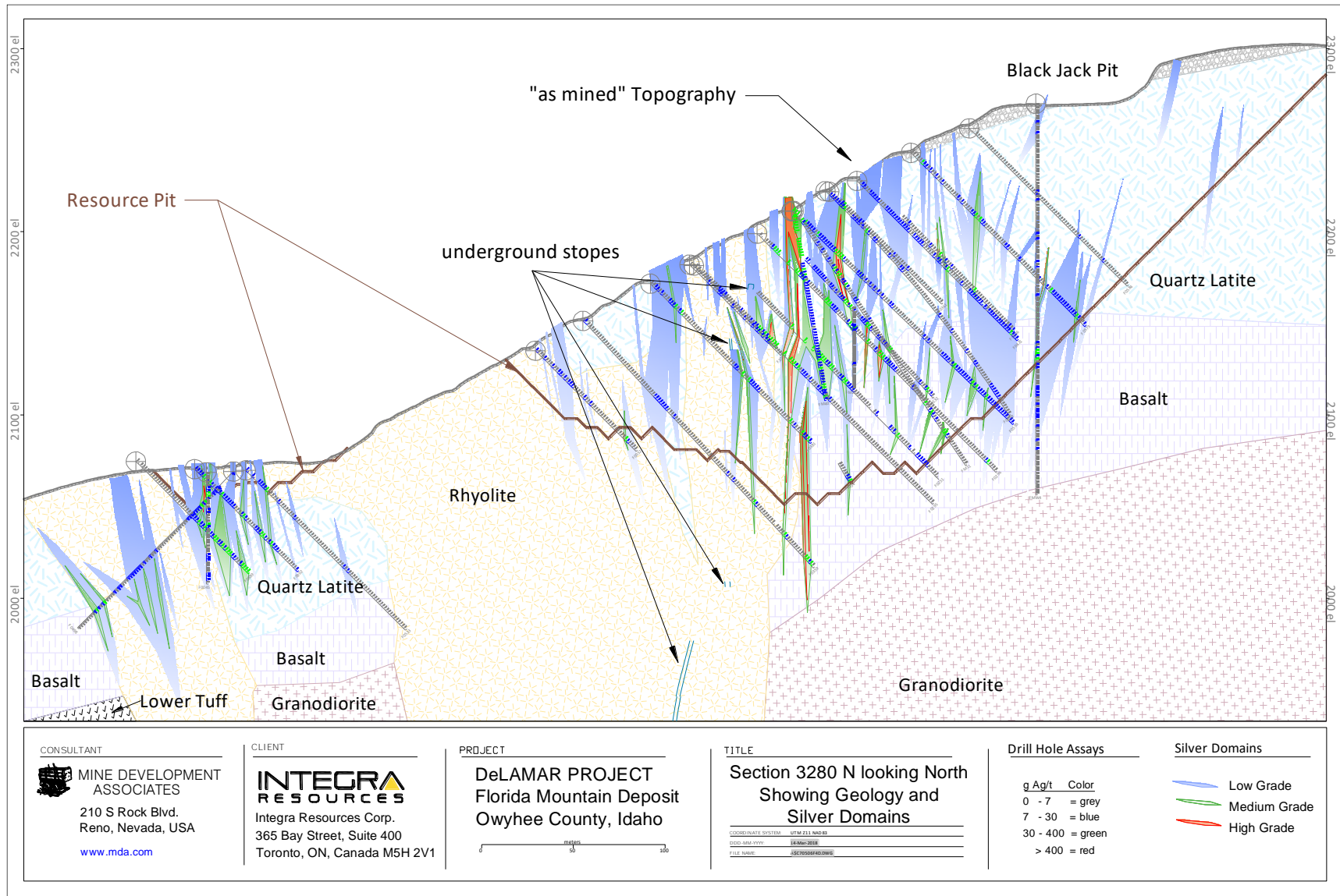
Figure 14.10 Cross Section 3280 N, Geology and Silver Domains for the Florida Mountain Area
